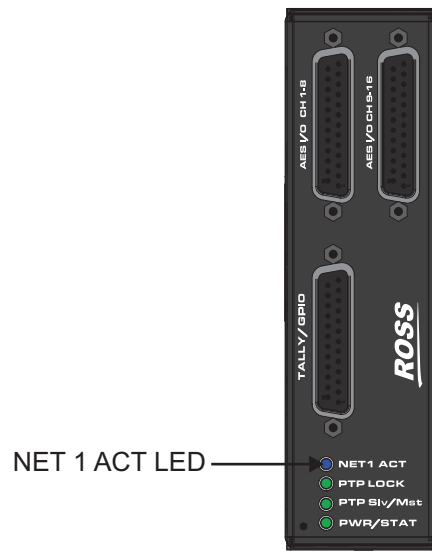
Figure 8 IGGY-AES16.16 — NET 1 ACT LED
