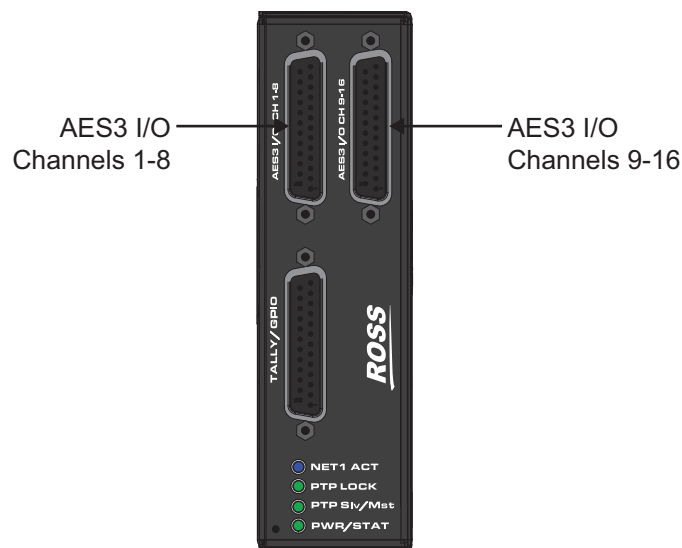
Figure 9 IGGY-AES16.16 — AES3 I/O Connectors
