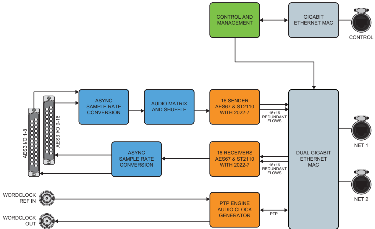
Figure 1 IGGY-AES16.16 Work Flow Diagram
