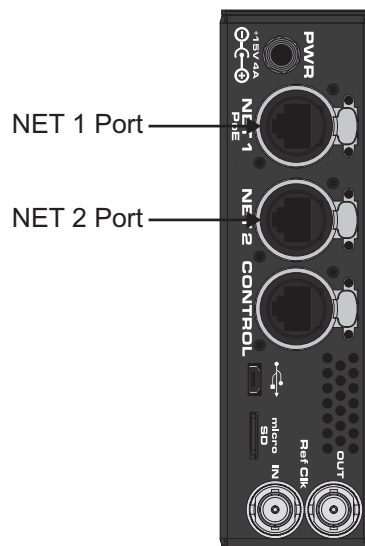
Figure 7 IGGY-AES16.16 — NET Ports
