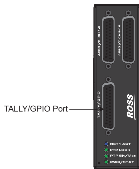
Figure 12 IGGY-AES16.16 — TALLY/GPIO Port
