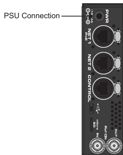
Figure 4 IGGY-AES16.16 — PWR Connection
