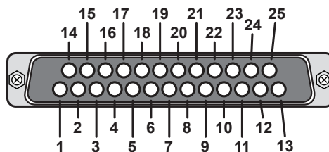
Figure 18 TALLY/GPIO Port — Pin-out Designations
