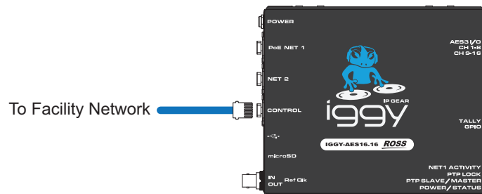
Figure 15 IGGY-AES16.16 Cabling — CONTROL Port
