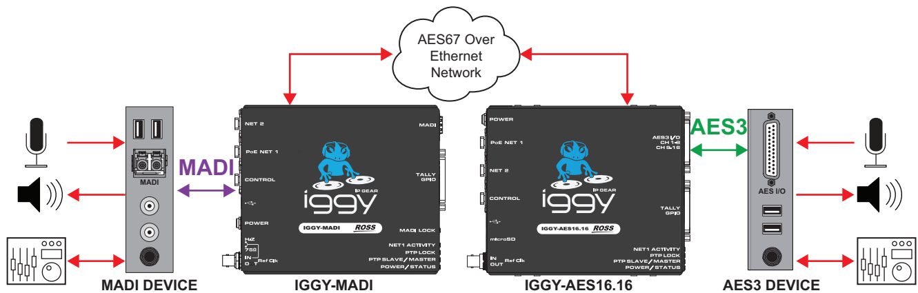
Figure 2 Possible Workflow with an IGGY-MADI and an IGGY-AES16.16
