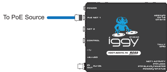
Figure 13 IGGY-AES16.16 Cabling — PoE Port
