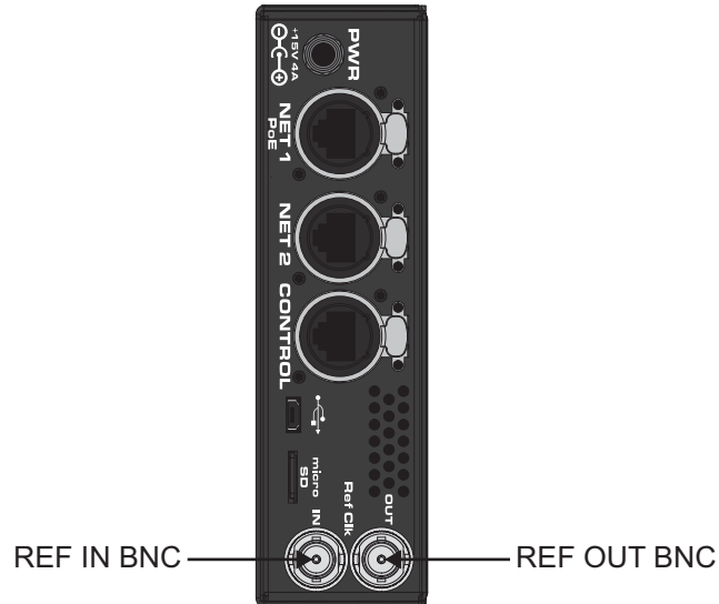
Figure 10 IGGY-AES16.16 — Reference Connections
