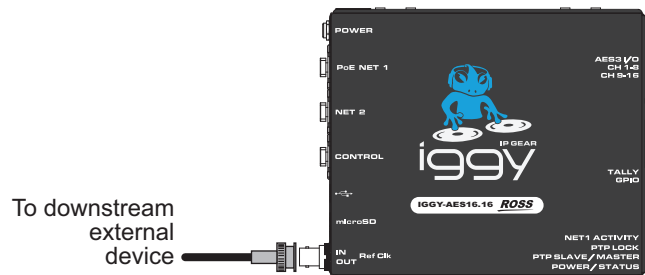
Figure 16 IGGY-AES16.16 Cabling — REF OUT
