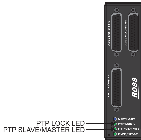
Figure 11 IGGY-AES16.16 — PTP Status LEDs
