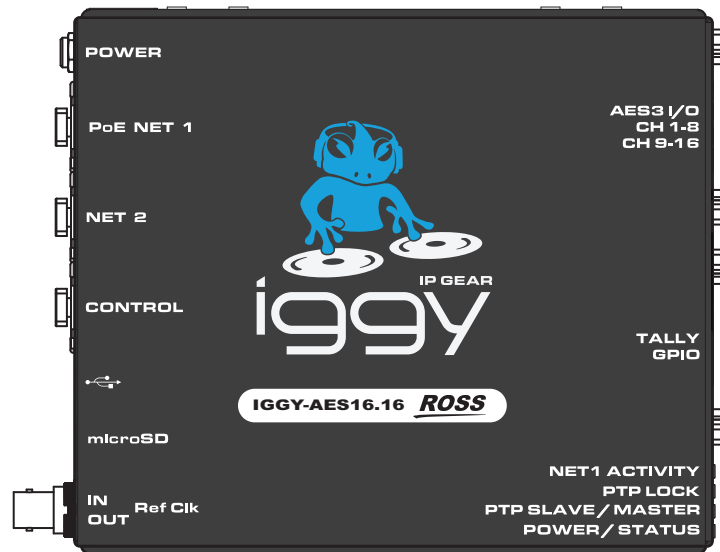
Figure 3 IGGY-AES16.16 — Faceplate Components
