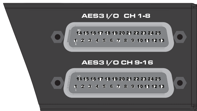
Figure 17 IGGY-AES16.16 Cabling — AES3 I/O Pinouts
