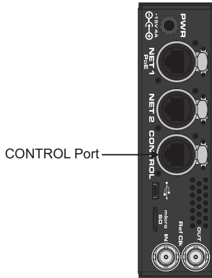
Figure 6 IGGY-AES16.16 — CONTROL Port
